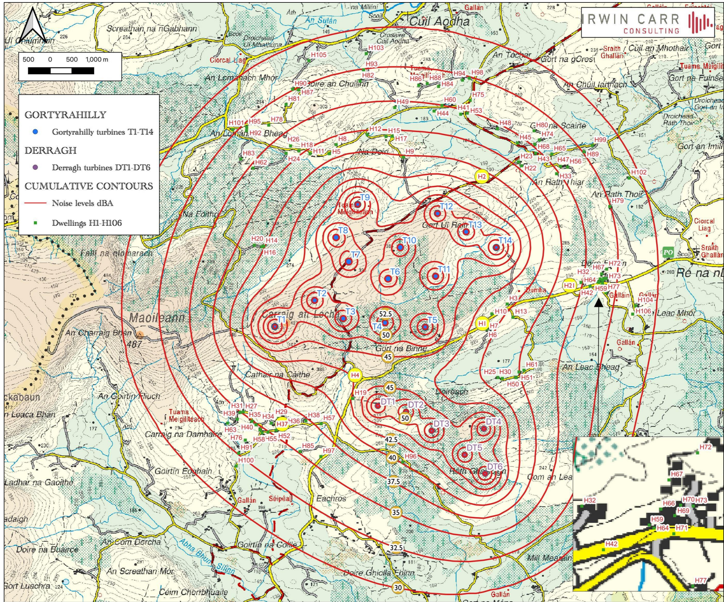
Figure 11.2: Cumulative noise map (Gortyrahilly + Derragh) at 8m/s wind speed with each contour line representing a 2.5dBA change in noise level
